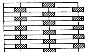
10 1 header; 2 stretchers alternating coursewise
